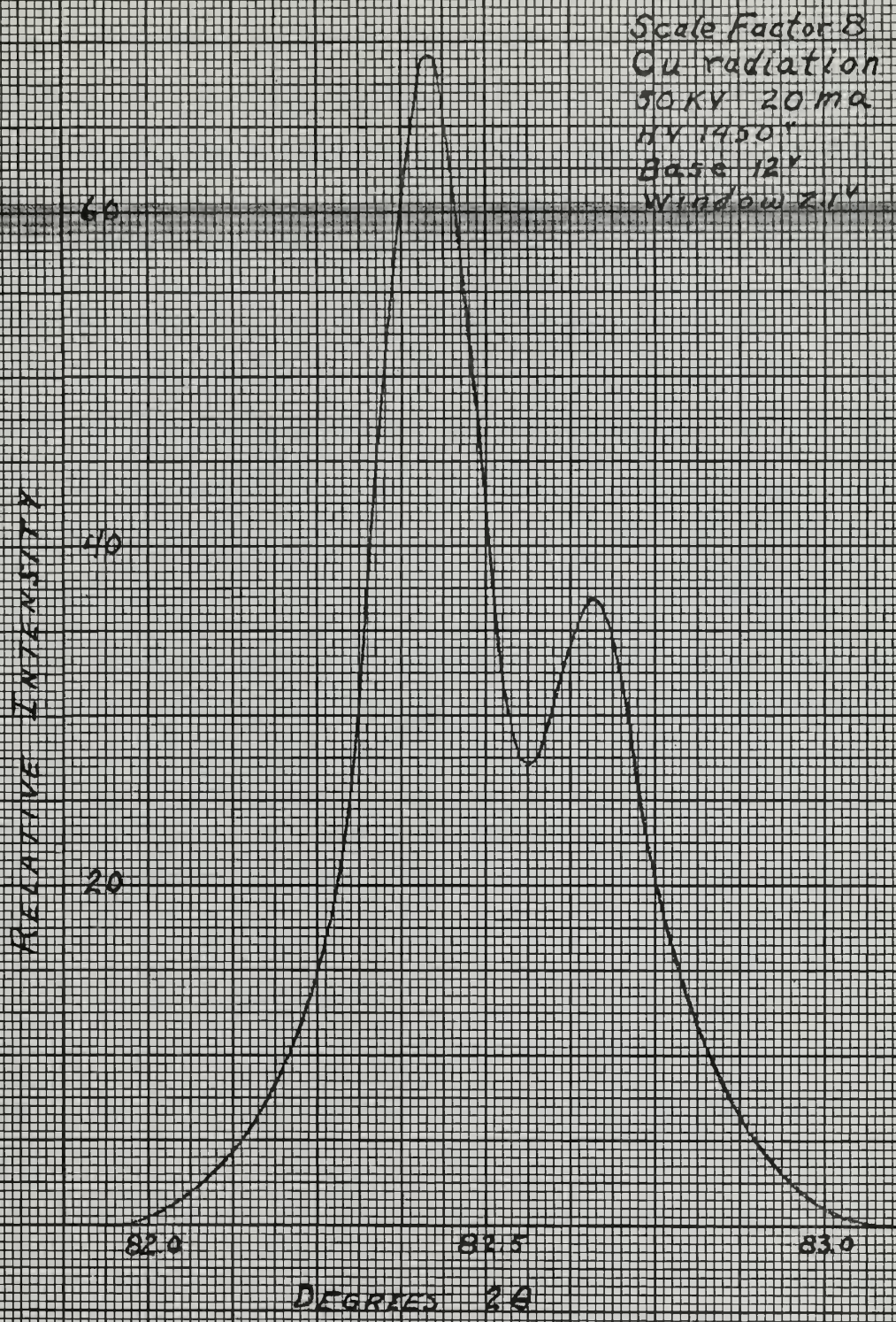
Figure 8 (112) \alpha Peak Brittle Specimen
